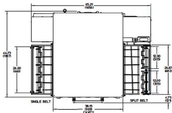
PS638E-V Top View
